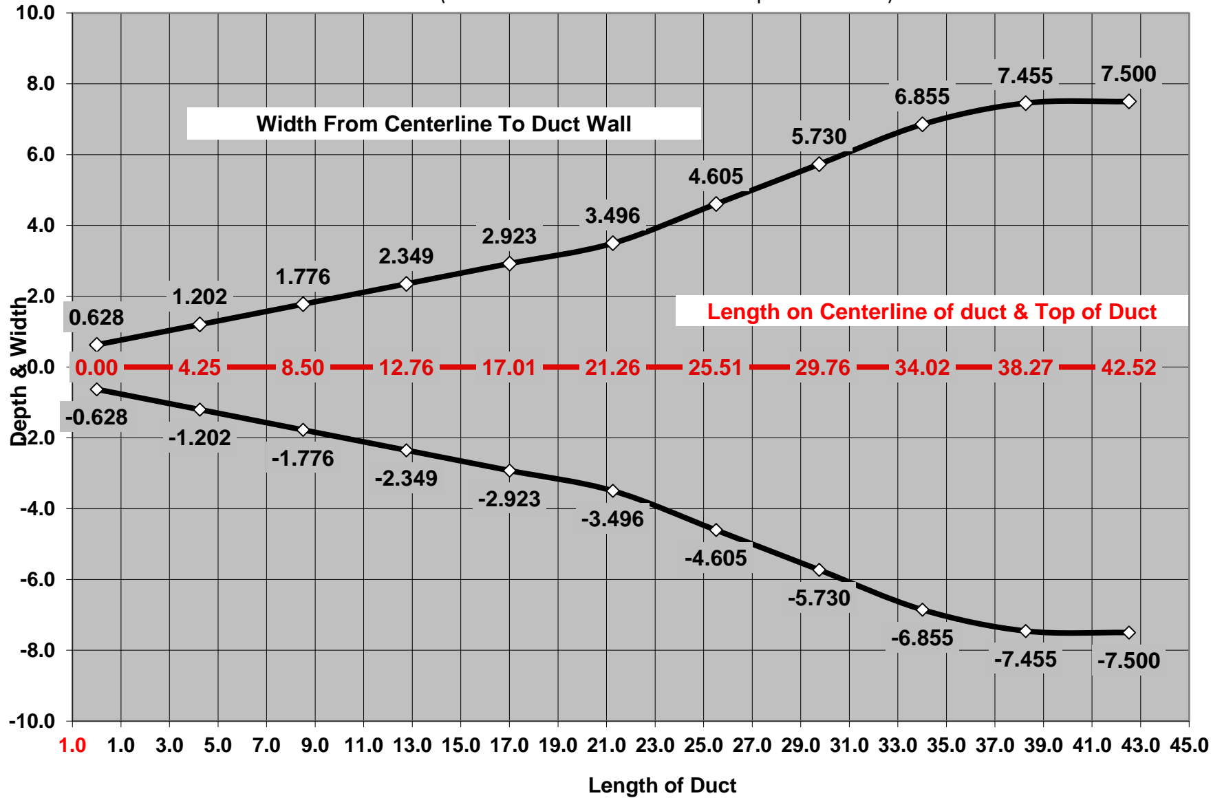
NACA Duct Co-ordinates (derived from curve fits of several optimized ducts)
